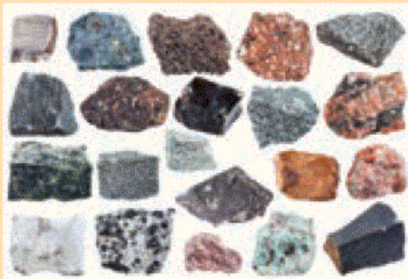
Fig. 2. Rocile magmatice
