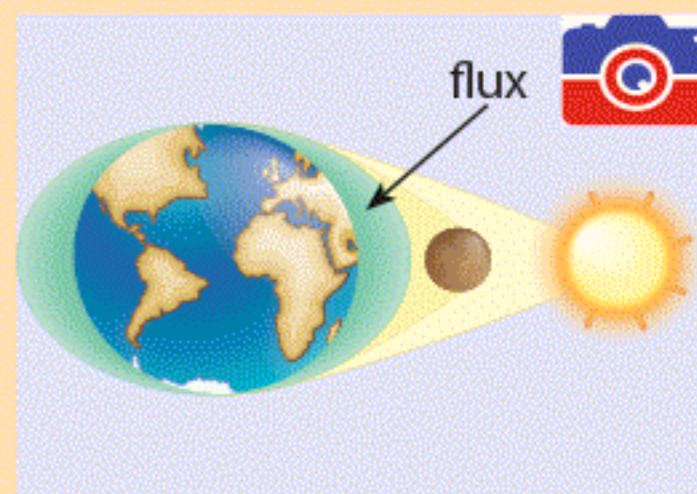
Fig. 7. Producerea mareelor
